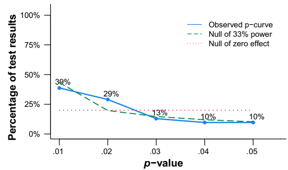
Fig. 10. Default plot produced by p -curve for sample of studies in which the effect of interest is a moderator of syntactic priming. The solid line is the distribution of p -values in the study. The dotted line shows the expected distribution of p -values if there was no underlying effect. The dashed line shows the expected p -curve under 33% statistical power. The right skew in the solid line shows there is evidential value in this set of studies.
